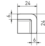
Außenecke | outside corner | GTVR4... | GTVR4F... | 24×24×24 mm
